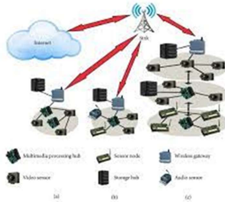
Fig. 2.4.1: Route Discovery in Industrial Wireless Sensor Networks
